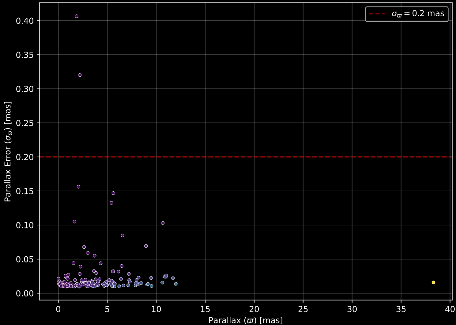
APOGEE DR17 Field: [110+60] Parallax Quality (n= 182)
