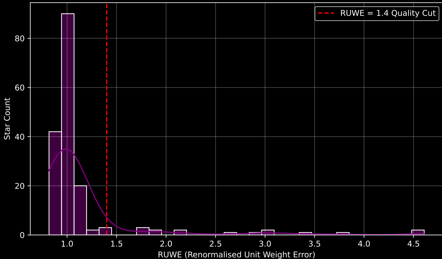
GAPOGEE DR17 Field [110+60] RUWE Distribution (n= 172)
