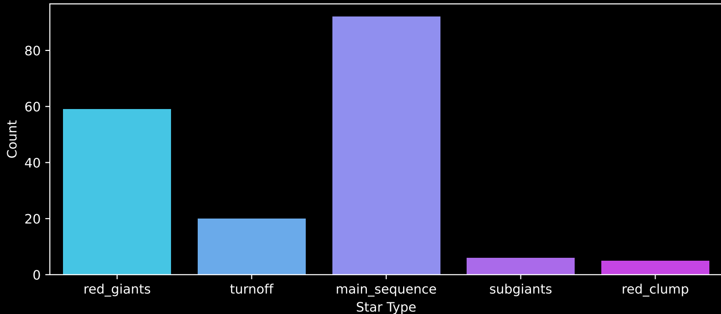
APOGEE DR17 Field: [110+60] Count plot of Star Type
