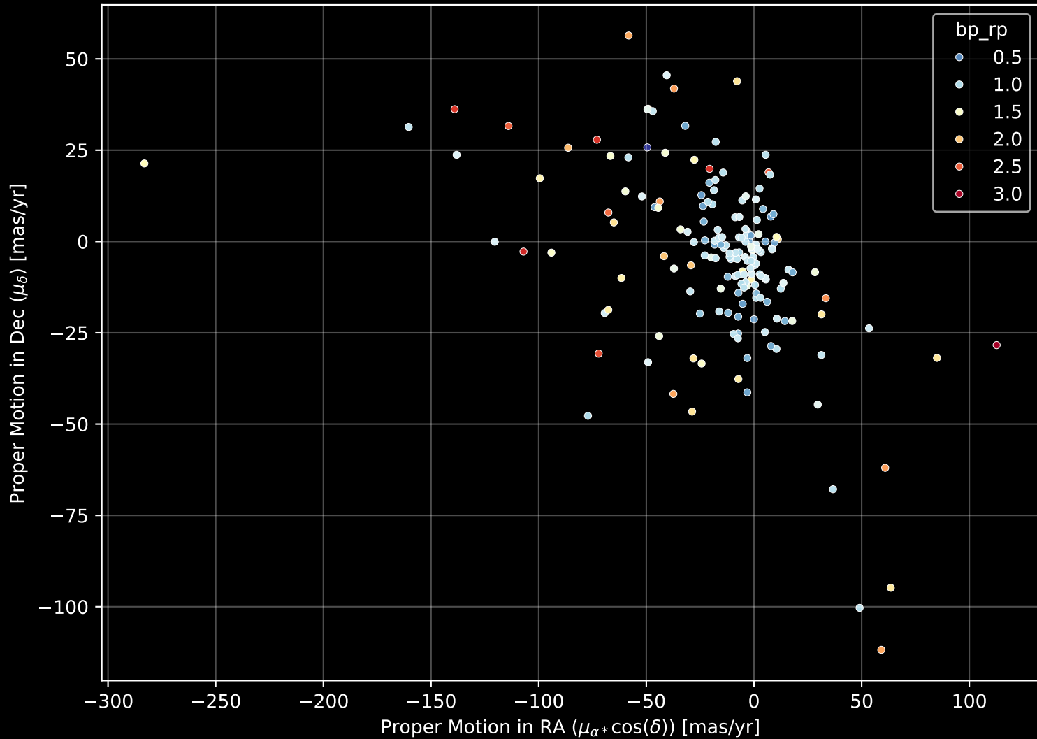
APOGEE DR17 Field: [110+60] Proper Motion Diagram (n= 182)
