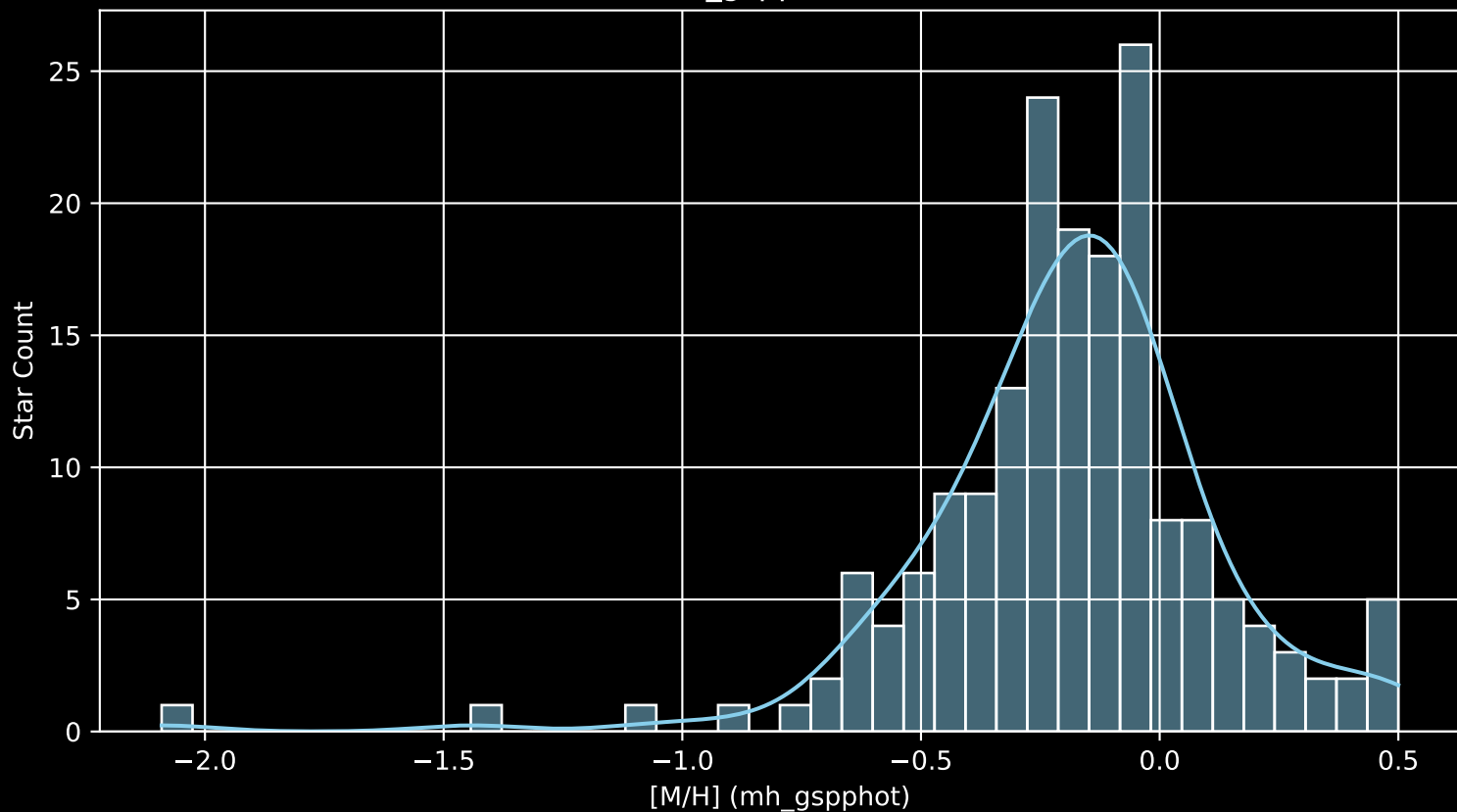
APOGEE DR17 Field: [110+60 [M/H] (mh_gspphot) (n= 178)
